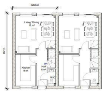
05 Ground Floor Plan 1 : 100
