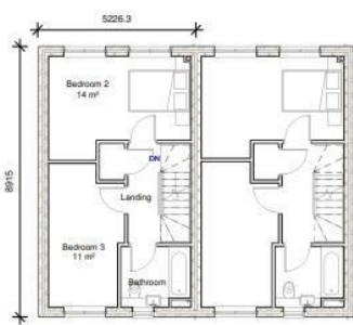
06 First Floor Plan 1 : 100
